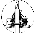
DN250 / DN300 Packing Detail Salmastra Detayı
