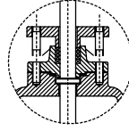
DN350 / DN1000 Packing Detail Salmastra Detayı
